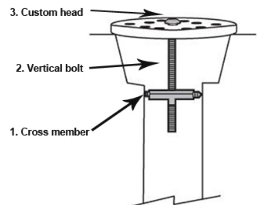
Lock and Stop Diagram (side view of drain)
